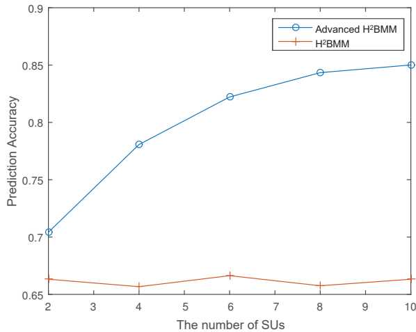
Figure 11. Prediction accuracy of Advanced H 2 BMM and H 2 BMM
