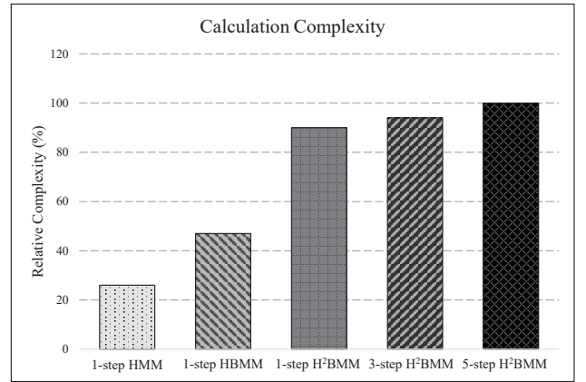
Figure 9. Computation Complexity of HMM, HBMM and H 2 BMM
