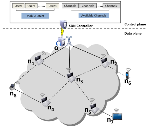
Fig. 2. Software-defined VDN model
