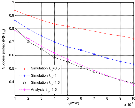
Figure 4: The success probability of MDCR mechanism with the carrier sensing threshold \gamma
