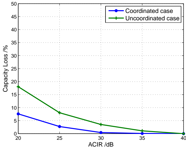
Figure 2: NB-IoT aggressor, cdma2000 victim (DL)
