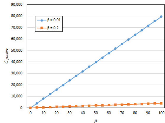
Figure 7. Packet data transmission overhead ( \mu = 0.1 ).
