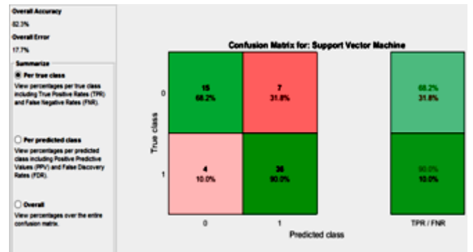
Figure 4. Confusion Matrix of Proposed Classification, using PCA-Based for Classification
