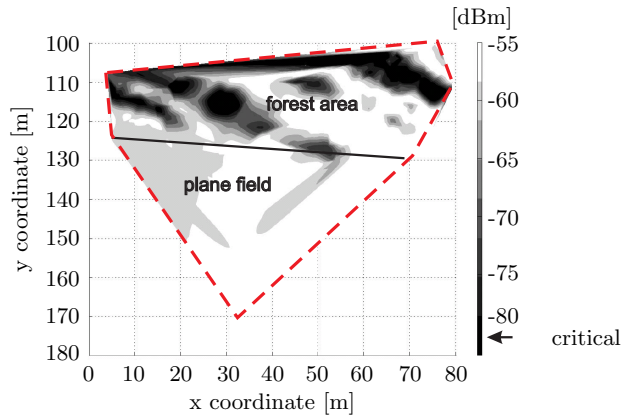
Figure 7: Distribution of Received Signal Strength
