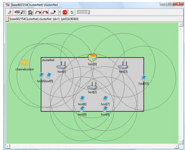
Figure 4. Example of Cluster-Tree topology
