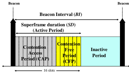
Figure 1. Example of the IEEE 802.15.4 Superframe structure.
