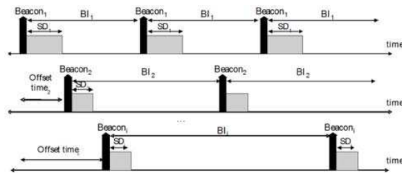
Figure 2. Collision avoidance by distributing the SDs .
