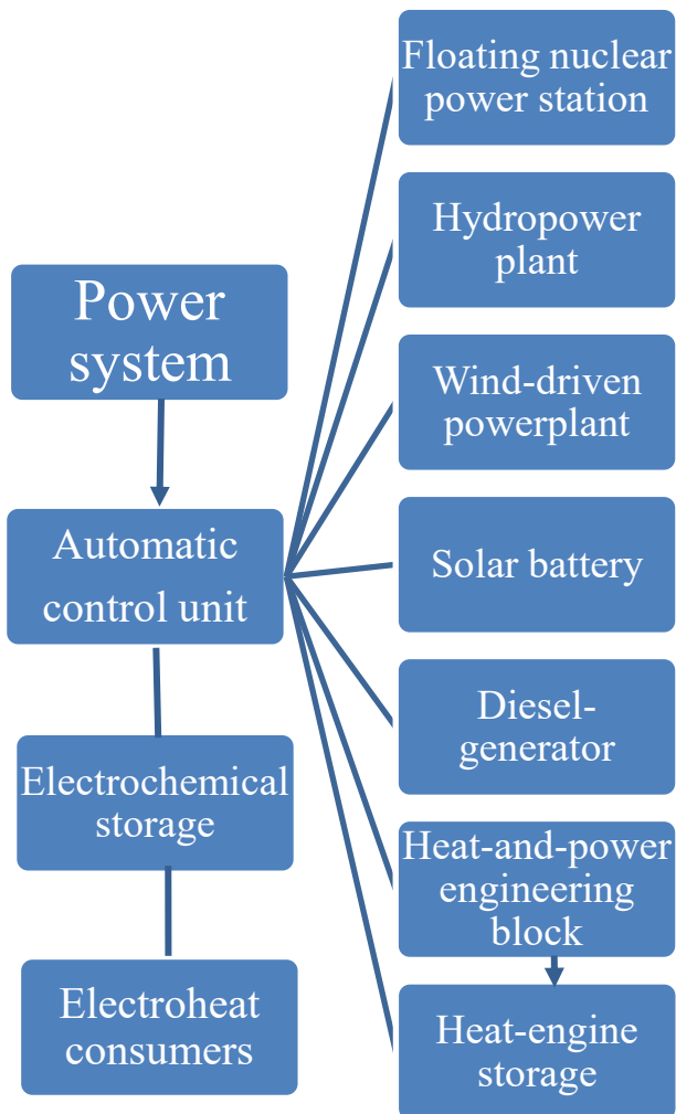
Figure 1. The combined electro heat supply of consumers
