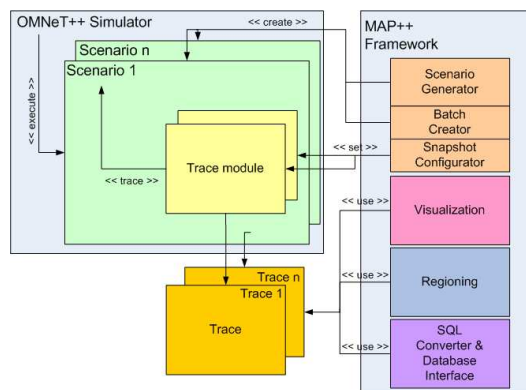
Figure 1: MAP++ Architecture
