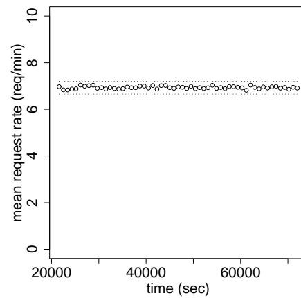
Figure 4: Average requests per server per minute using uniform server popularity distribution
