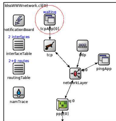
Figure 1: The StandardHost and its submodules. HttpBrowser and HttpServer components plug in as tcpApps .
