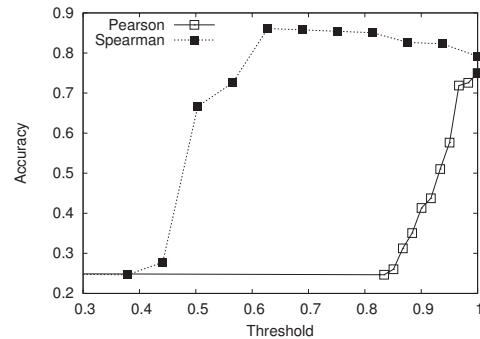
Figure 4: Accuracy comparison
