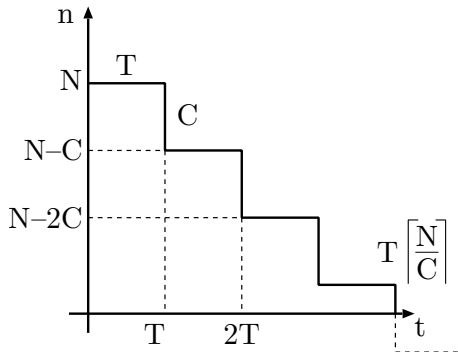
Figure 2: Fluid evolution: Deterministic task execution time
