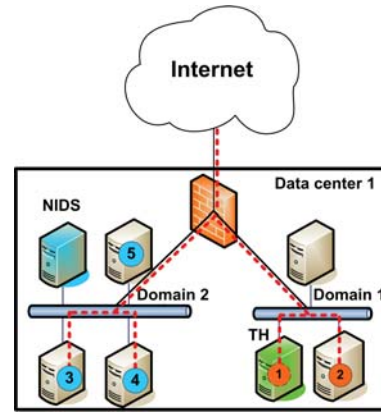
Figure 5: Motivational scenario for security-aware VNE
