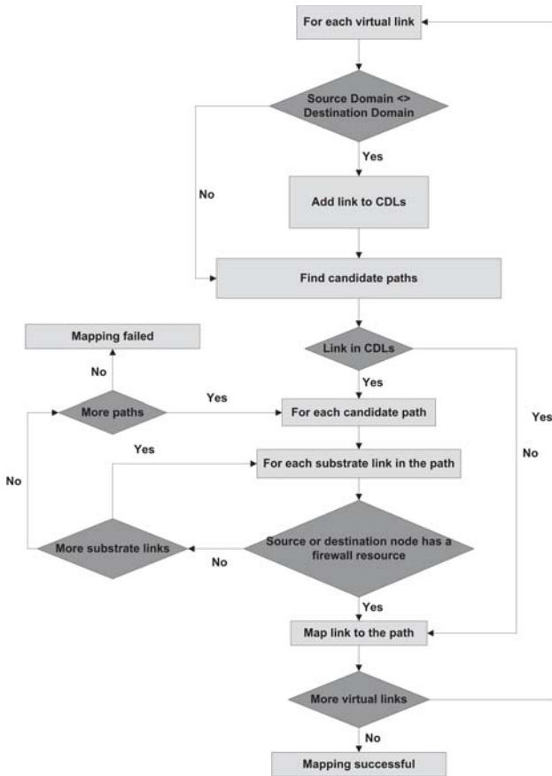
Figure 4: Embedding algorithm for CDLs
