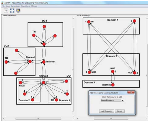
Figure 6: Adding a firewall-resource to ALEVIN
