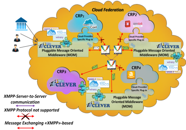
Figure 4: Technical Realization of the CADS Architecture
