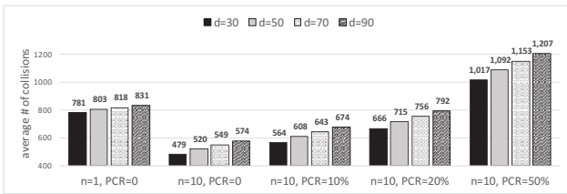
Figure 12: Average Number of Collisions among Molecular Packets Fragmented from 100 Information Molecules
