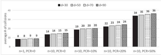
Figure 9: Average Number of Collisions among Molecular Packets Fragmented from 10 Information Molecules
