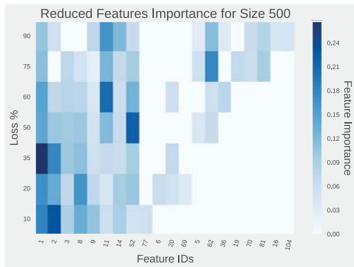
Figure 7: (a) Feature significance in size 500 networks for all loss models and reduced feature sets. The darker the color the higher the feature significance. Additionally, numbers are included to indicate feature rank; higher is better.
