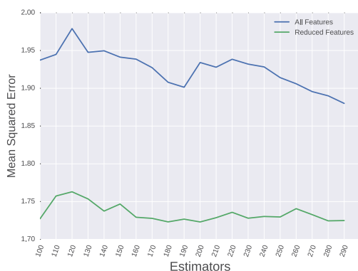
Figure 3: Mean squared error (MSE) for different number of Random Forest estimators for networks of size 300 and heavy channel loss (90%). A lower MSE here indicates a better performance.
