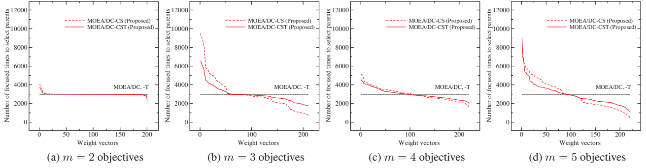
Figure 8: The total number of focuses on each weight vector for offspring generations on WFG4 with k = 2
