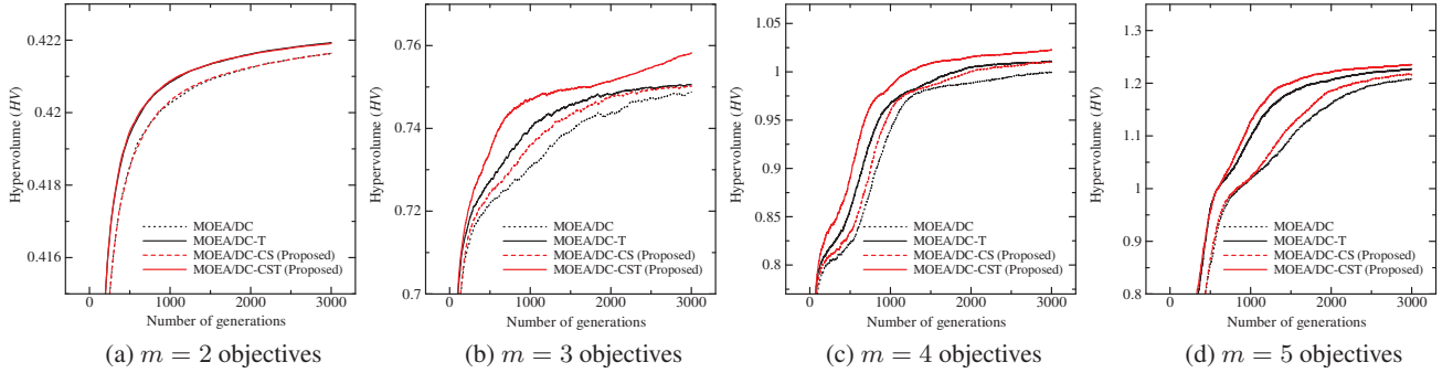
Figure 4: Transition of HV on WFG4 with the problem difficulty parameter k = 10
