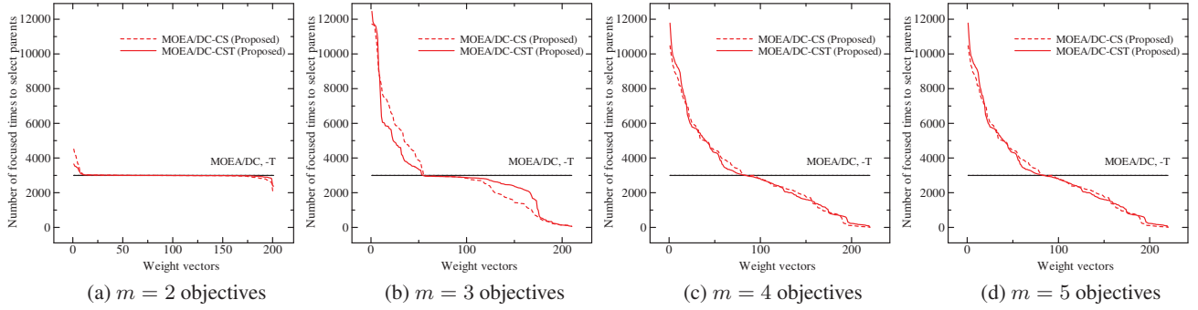
Figure 10: The total number of focuses on each weight vector for offspring generations on WFG4 with k = 10
