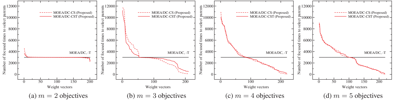
Figure 9: The total number of focuses on each weight vector for offspring generations on WFG4 with k = 6
