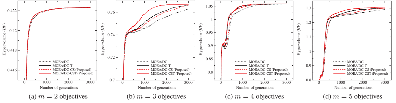
Figure 2: Transition of HV on WFG4 with the problem difficulty parameter k = 2
