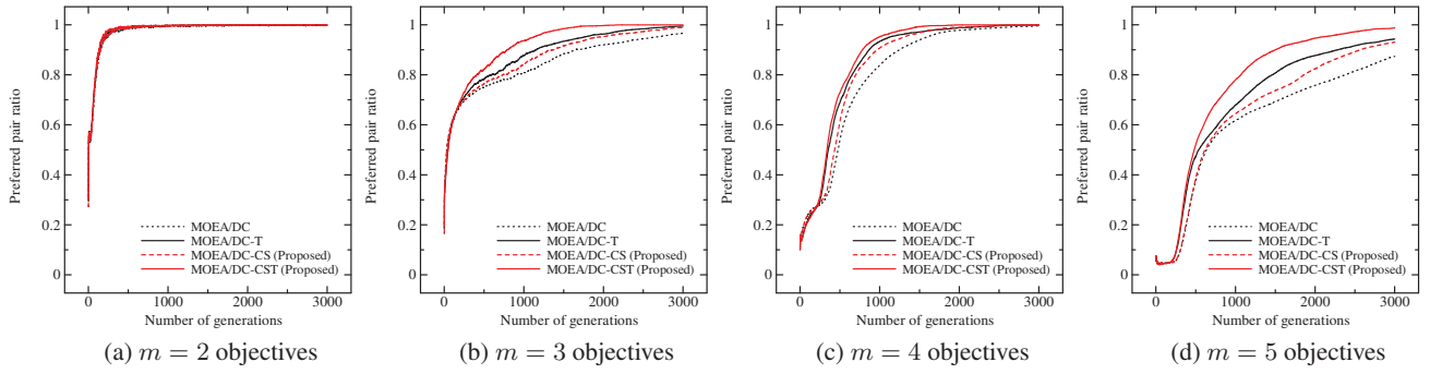
Figure 5: Transition of well-matched pair ratio among all pairs of weight vector and solution on WFG4 with k = 2
