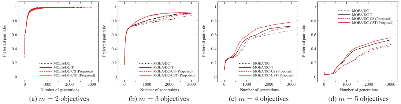
Figure 7: Transition of well-matched pair ratio among all pairs of weight vector and solution on WFG4 with k = 10
