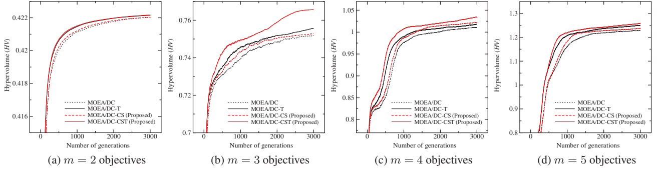
Figure 3: Transition of HV on WFG4 with the problem difficulty parameter k = 6
