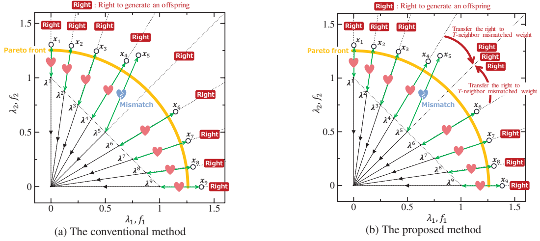
Figure 1: Rights to generate offspring for well-matched and mismatched pairs of weight vector and solution
