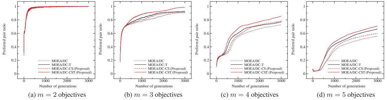
Figure 6: Transition of well-matched pair ratio among all pairs of weight vector and solution on WFG4 with k = 6
