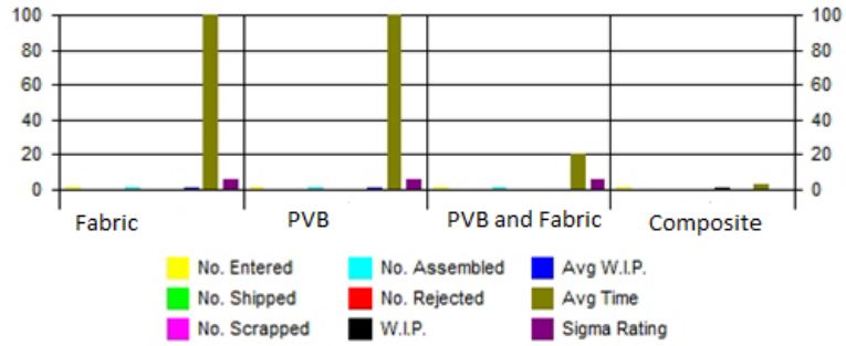
Figure 5. Machine statistic
