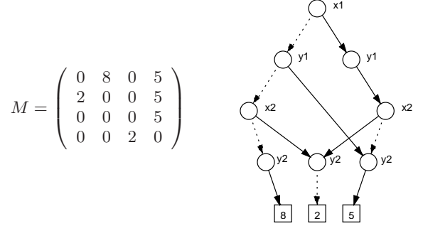
Figure 6: A multi-terminal binary decision diagram (MTBDD) to encode a sparse matrix. The two binary variables x_1, x_2 encode the four row indices, while y_1, y_2 are responsible for the columns.
