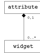
Figure 11: Attributes are connected with window interaction controls.
