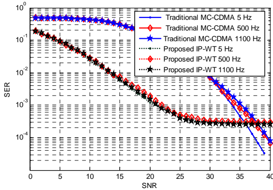
Figure 6. Performance of the proposed and traditional model in selective fading channel (Doppler frequencies are: 5, 500, and 1100 Hz, path delay=1 sample, path gain=-8 dB)
