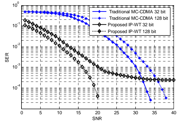
Figure 7. Performance of the proposed and traditional model in selective fading channel (Doppler frequencies are: 5 Hz, path delay=1 sample, path gain=-10 dB, code length=32, and 128 bit)
