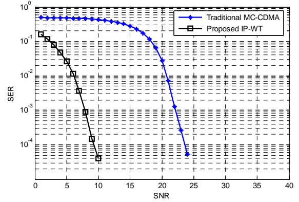
Figure 4. Performance of the proposed and traditional model in AWGN channel
