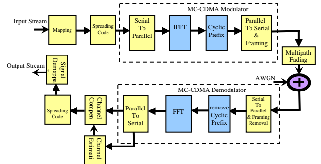
Figure 1. Traditional MC-CDMA model based FFT
