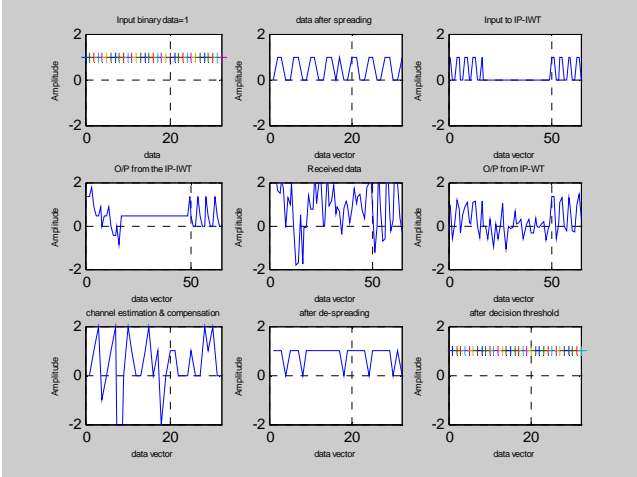
Figure 3. Time envelope of the proposed model
