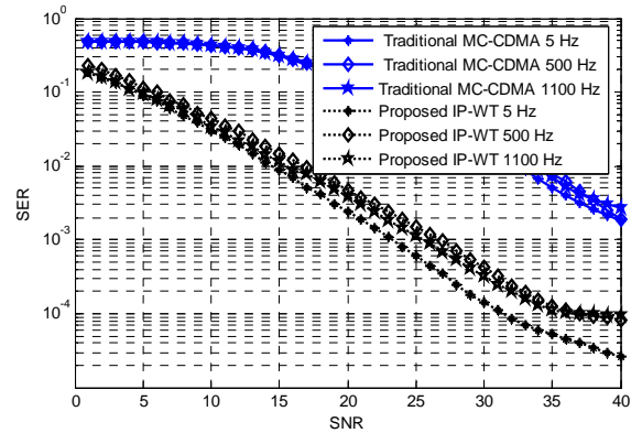
Figure 5. Performance of the proposed and traditional model in flat fading channel (Doppler frequencies are: 5, 500, and 1100 Hz)
