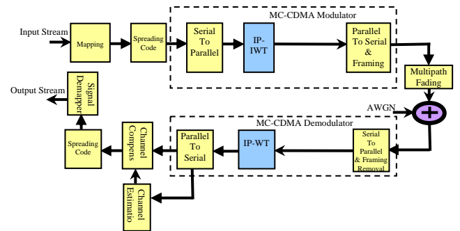
Figure 2. A proposed MC-CDMA model based In-Place wavelet transform
