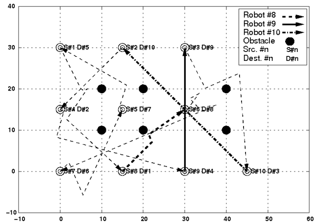
Figure 7. Robot initial positions and trajectories.
