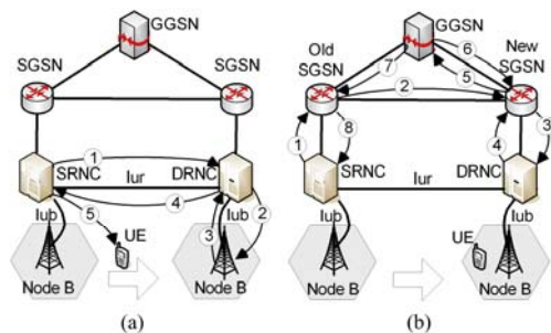
Figure 3. User mobility handling: (a) inter-RNS handover and (b) inter-SRNS relocation.
