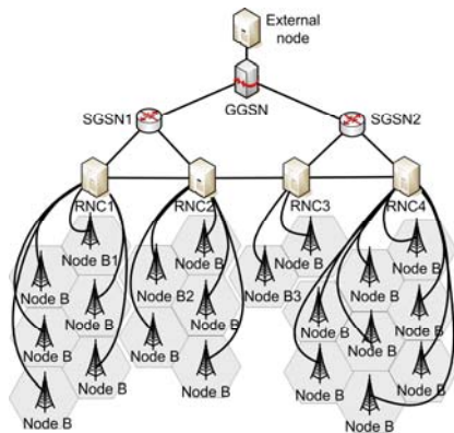
Figure 5. Simulation topology.
