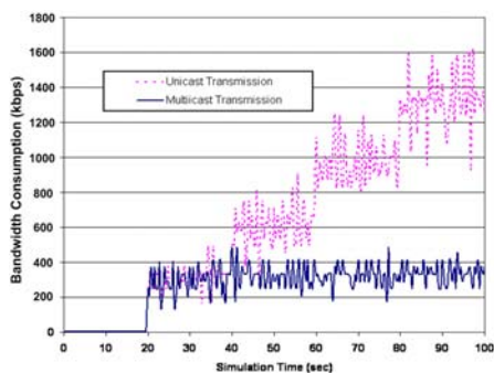
Figure 7. Multicast transmission over Iur interface.
