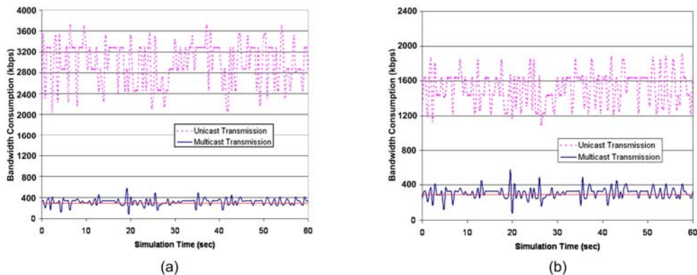
Figure 6. Bandwidth consumption in: (a) GGSN-SGSN1 and (b) SGSN1-RNC1 links.
