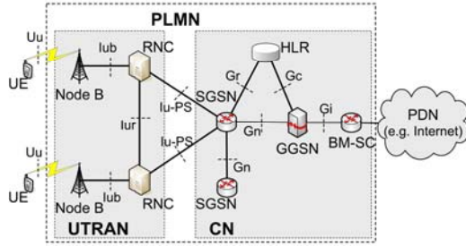
Figure 1. UMTS architecture for MBMS service.
