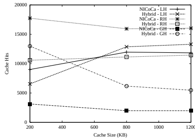
Figure 7: Impact of cache size on hits (small multimedia files and Zipfian access) in a very dense WMSN ( d = 10 ).
