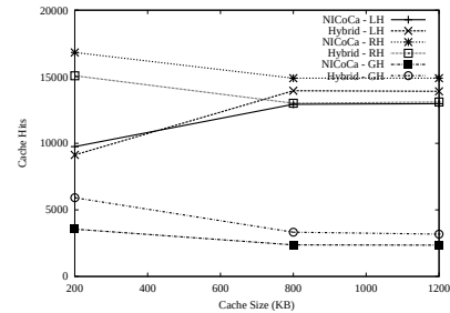
Figure 5: Impact of cache size on hits (small multimedia files and Zipfian access) in a sparse WMSN ( d = 4 ).
