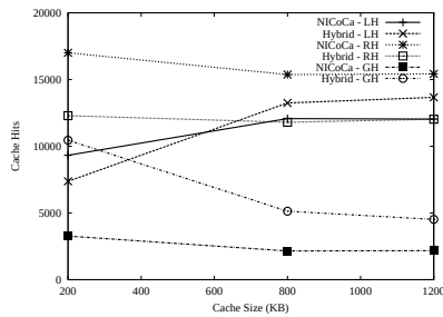
Figure 6: Impact of cache size on hits (small multimedia files and Zipfian access) in a dense WMSN ( d = 7 ).
