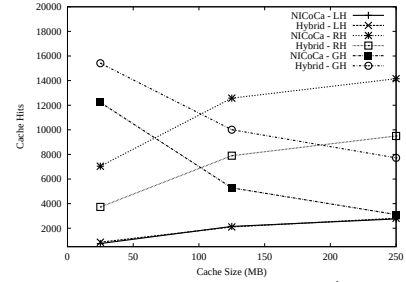
Figure 3: Impact of cache size on hits (large multimedia files and uniform access) in a dense WMSN ( d = 7 ).
