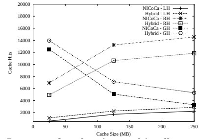
Figure 2: Impact of cache size on hits (large multimedia files and uniform access) in a sparse WMSN ( d = 4 ).
