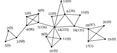
Figure 1: Calculation of \mathcal{NI} for a sample graph. The numbers in parentheses denote the \mathcal{NI} index of the respective node considering the whole WMSN topology.
