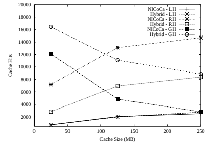
Figure 4: Impact of cache size on hits (large multimedia files and uniform access) in a very dense WMSN ( d = 10 ).
