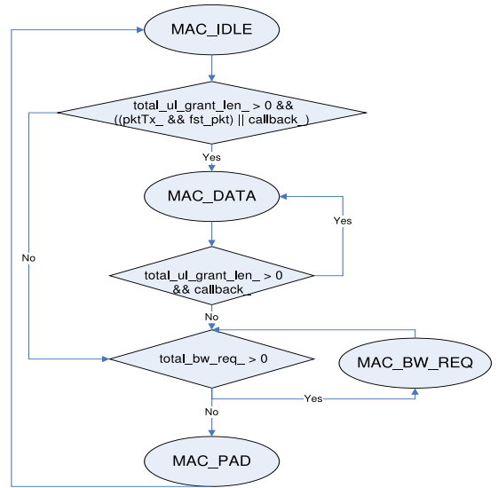
Figure 7: MacSS transmission states diagram
