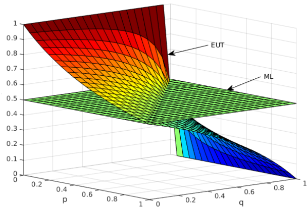
Figure 1: Decision surface for EUT and ML classifier.
