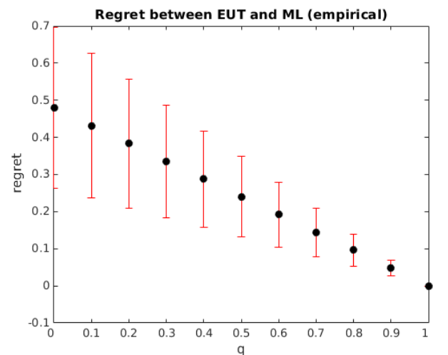
(c) Variation of Regret w.r.t. q (for p = 0.4 )
