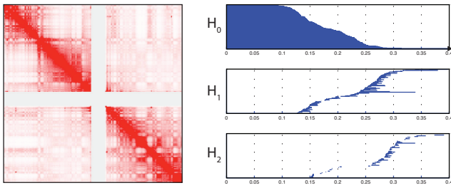
Figure 6: Hi-C data chromosome 1 from GM06690 human cell line data, from [9]. Left: Contact map representation. Right: PH identifies complex multiscale topology.
