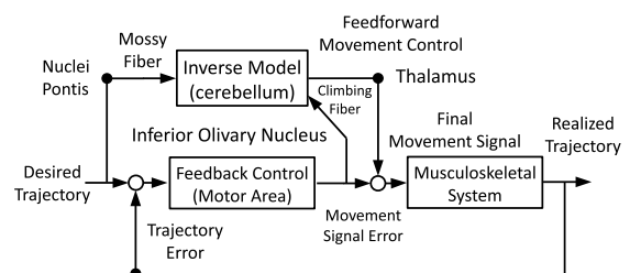
Figure 1: Structure of the internal model
