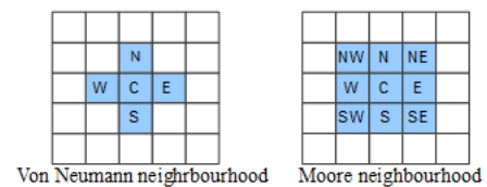
Figure 1. Two commonly used CA neighbourhoods: The Von Neumann neighbourhood (left) consists of the central cell itself plus 4 adjacent cells, and Moore neighbourhood (right) in which there are 8 adjacent cells.
