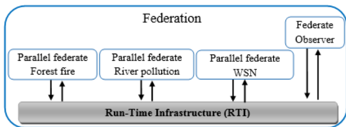
Figure 10. A federation of four federates: River, forest, WSN, and observer.
