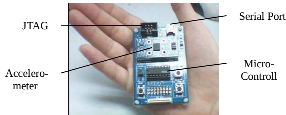
Figure 1. A snapshot of hardware system
