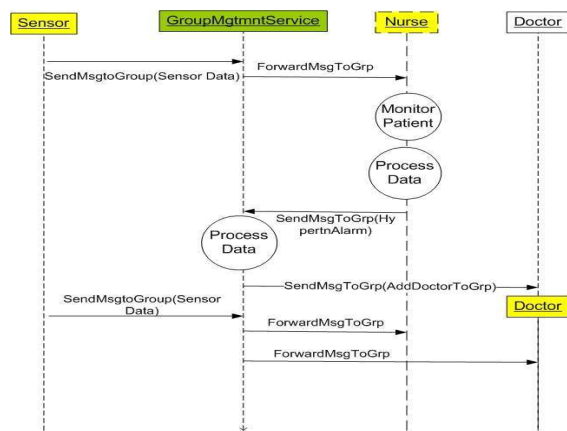
Figure 9. Group Reconfiguration Flow
