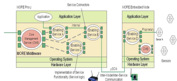
Figure 2. MORE Middleware Architecture
