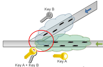
Fig. 3. Key management scenario: an intersection between areas where different keys are used. Vehicles in the red circle must know both Key A and Key B
