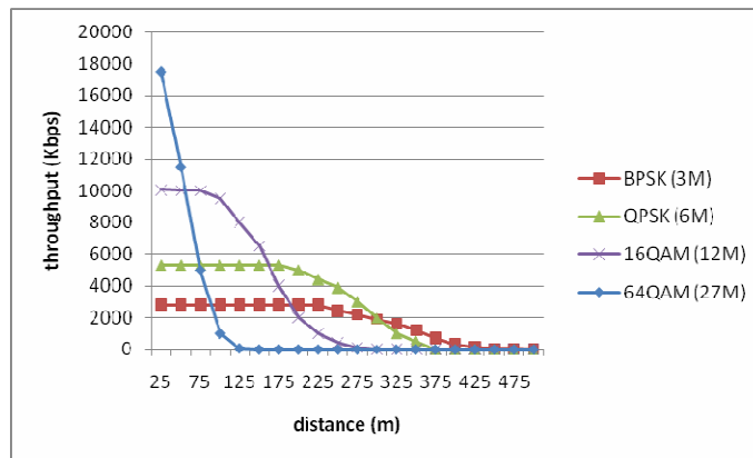
Figure 7: Theoretical throughput using different modulation over various distances
