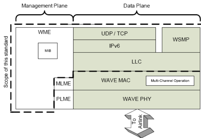
Figure 1: WAVE protocol stack. WAVE accommodates two protocol stacks: the standard Internet Protocol (IPv6) and the unique WAVE short message protocol (WSMP)
