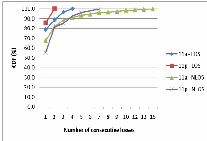
Figure 6: The cumulative distribution function for consecutive losses and the number of occurrences.
