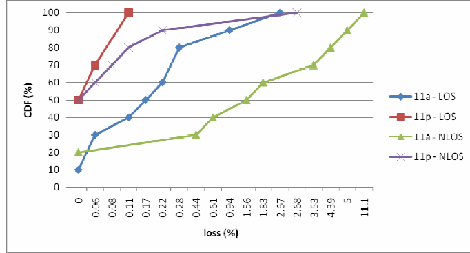
Figure 5: The distribution of consecutive packet losses
