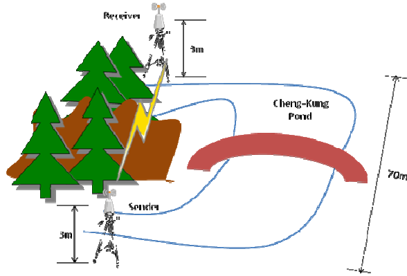
Figure 4: For the NLOS experiment, we measured at campus pond with a large rocky area and trees as an obstacle to introduce a multipath system.
