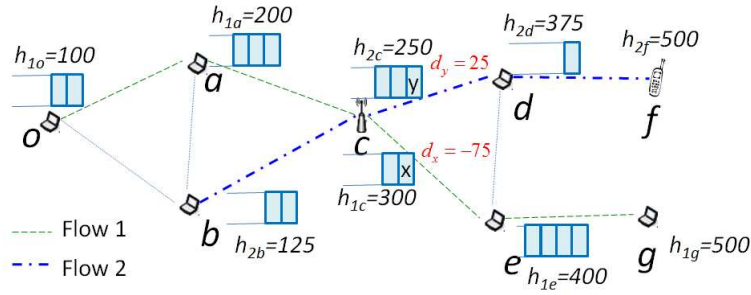
Fig. 3. An example illustrating the delay differential concept.
