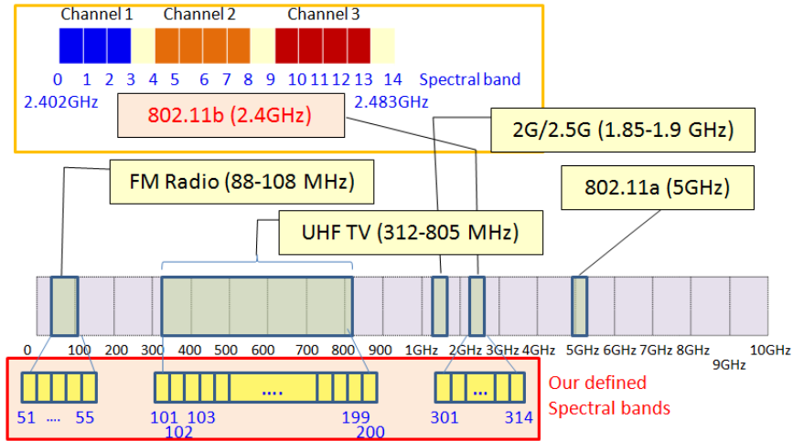
Fig. 2. The defined spectral bands marked with a serial number.
