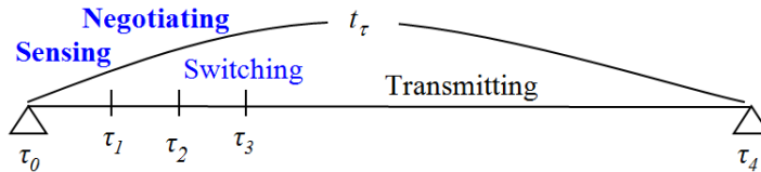
Fig. 1. A general operating cycle for a CRN.
