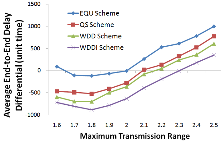
Fig. 6. The effect of transmission and sensing range on the average end-to-end delay differential.
