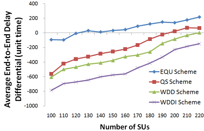
Fig. 7. The effect of the number of SUs on the average end-to-end delay differential.
