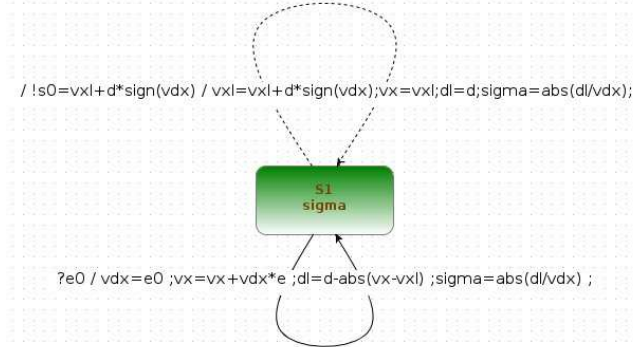
Figure 7: Quantized integrator
