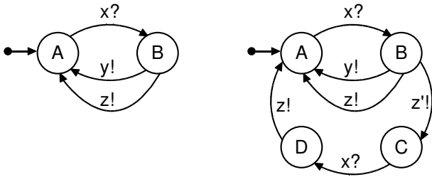
Figure 4: Behavioral Interface Automata
