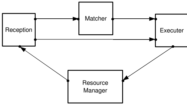
Figure 7: Exogenous Communication in ASK
