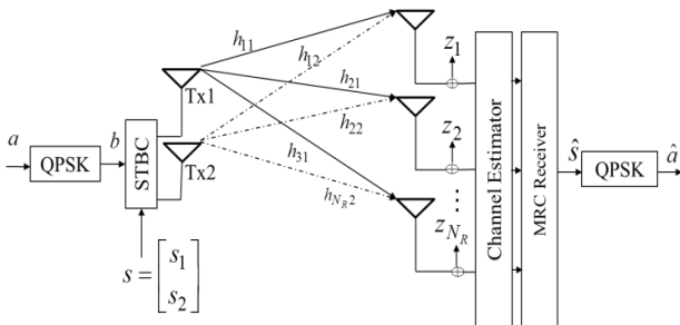
Figure 5: Architecture for Implementing STBC
