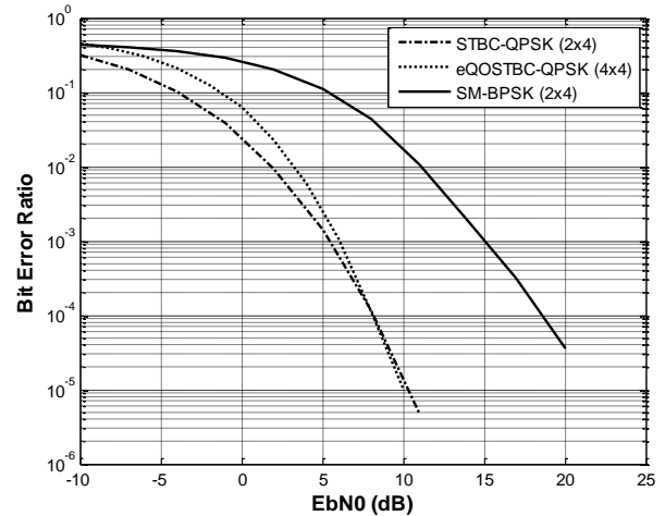
Figure 8: Comparison of two bits transmissions using SM, STBC and QOSTBC
