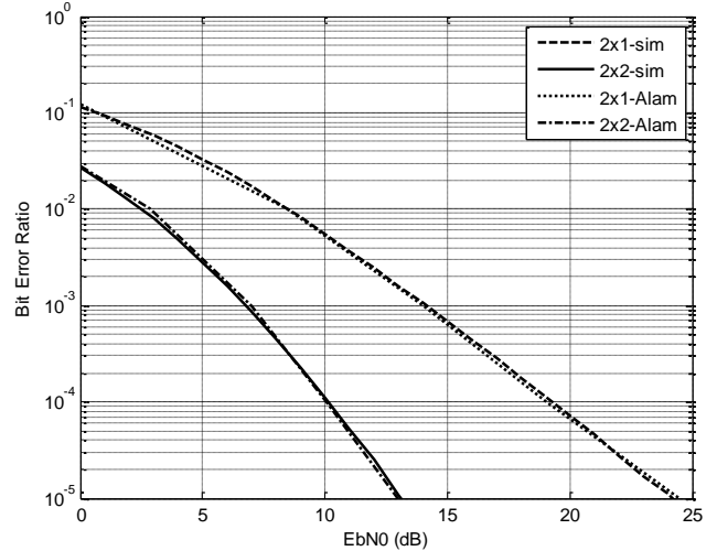
Figure 6: Results of 2×1 and 2×2 MIMO using STBC for the BPSK system
