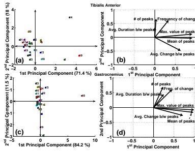
Figure 4: (a),(c): Global Analysis of tibialis anterior, and gastrocnemius; (b),(d): Respective loadings i.e. correlations between parameters and components.
