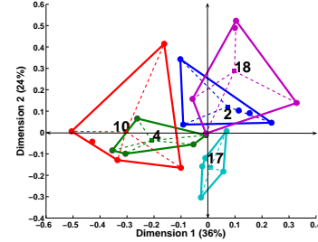
Figure 6: Compromise map of the participants with the performance of the sensors.
