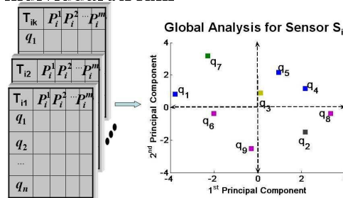
Figure 3: Construction of the global analysis space for the Sensor S_i .
