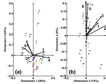
Figure 5: Analysis of compromise: Plot of the participants in the compromise space defined by dimensions 1-2(a) and 3-4(b) of the compromise matrix.
