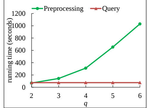
Fig. 1. Effect of Gram Length q
