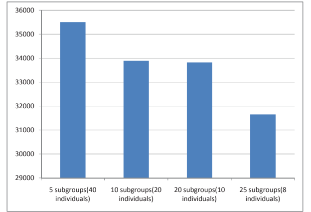
Fig. 6. the expected time of detection VS the number of subgroups
