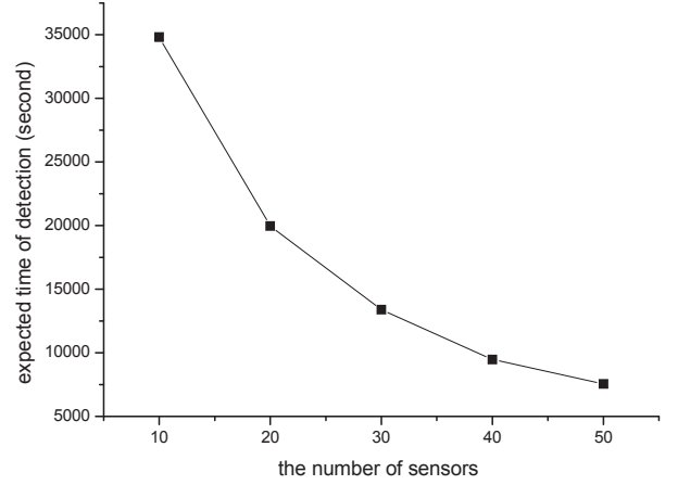
Fig. 5. expected time of detection VS the number of sensors
