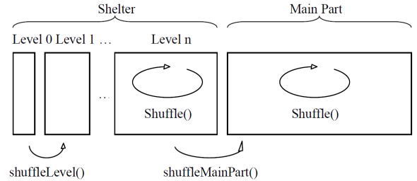
Fig. 2. Shuffle Algorithms Overview.
