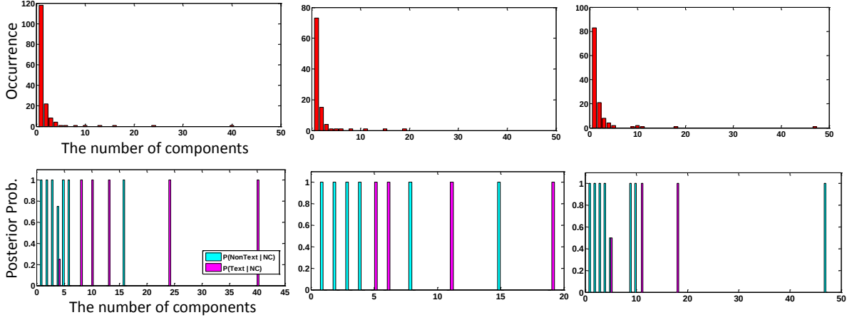
Figure 5. Histograms of the number of components and posterior probabilities
