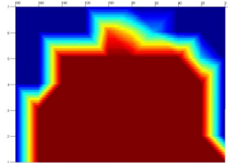
Figure 8: Accessible caption: Shows the average Detection Distance-Orientation Maps for Tag 1 on Material 1 using an external antenna. The red region in this figure is much larger than in the internal antenna case and extends outward up to 7 inches.
