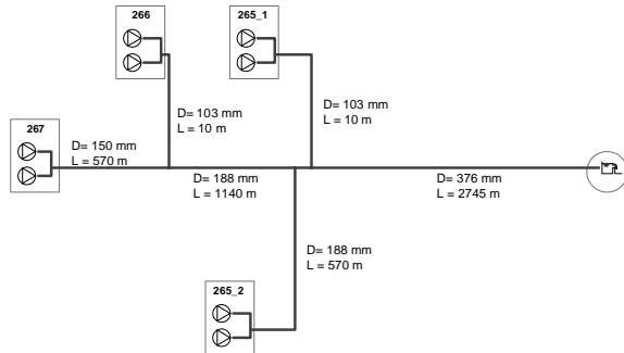
Figure 9. Schematisation of Almere Buiten-Oost system
