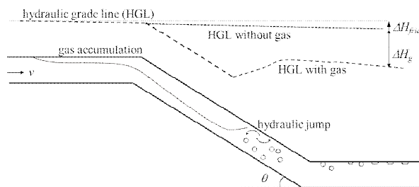
Figure 1. The effects of accumulating gas
