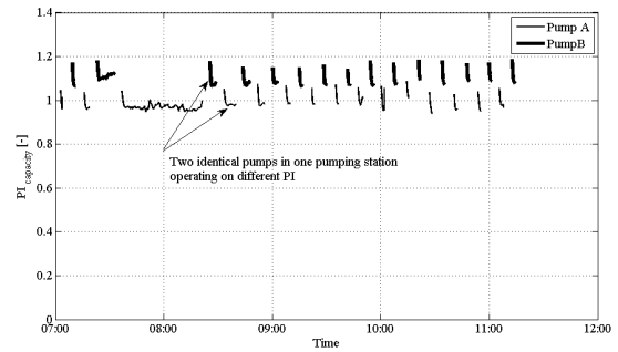
Figure 10. Different PIs for two identical pumps in one pumping station
