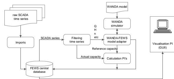
Figure 6. TAMTAM flowchart
