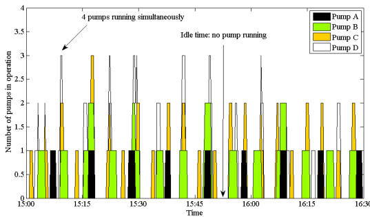
Figure 12. Pump operation in the afternoon
