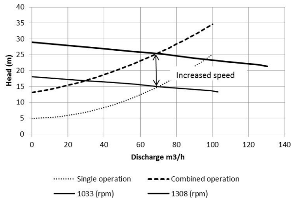
Figure 4. Different duty points for variable speed pump in single operation and combined operation
