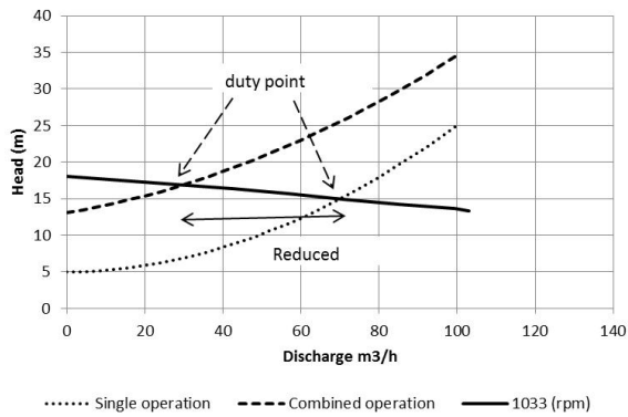
Figure 3. Different duty points for fixed speed pump in single operation and combined operation
