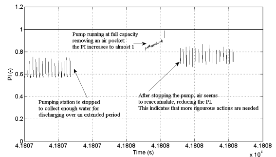
Figure 11. Release of air demonstrates the positive effect of PIs
