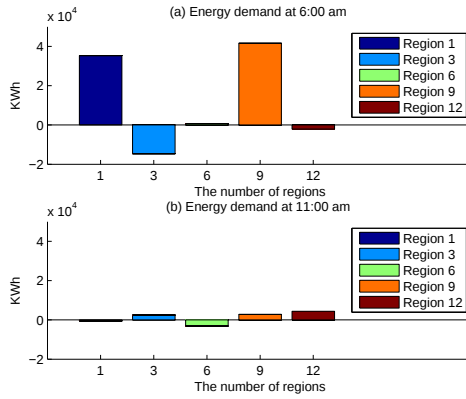
Fig. 6: Energy demand in the morning rush hours.
