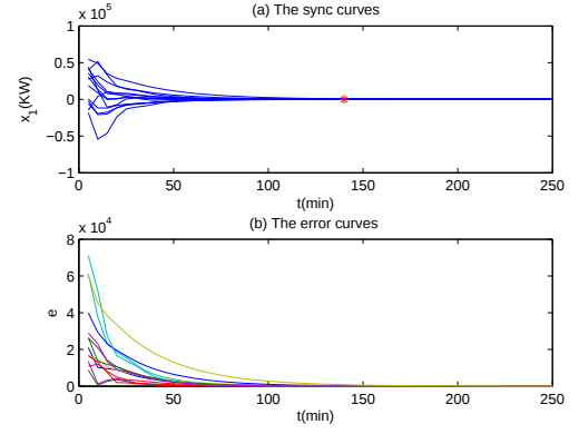
Fig. 4: Synchronization of the V2G network.
