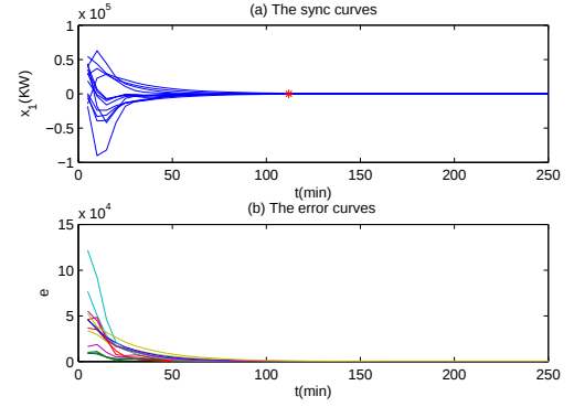
Fig. 5: Synchronization of V2G network at double trip-rate.
