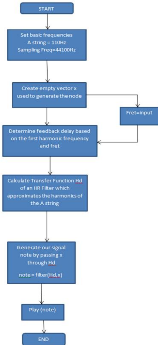
Figure 4. Flowchart- Sound module
