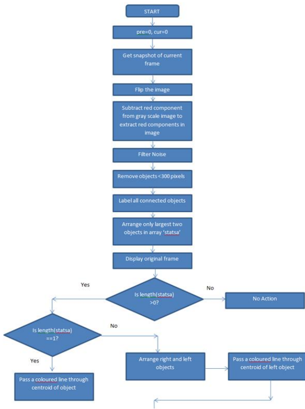
Figure 1. Project Flowchart-Part one
