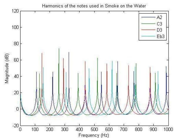
Figure 5. Harmonics of the notes used in 'Smoke on the Water'
