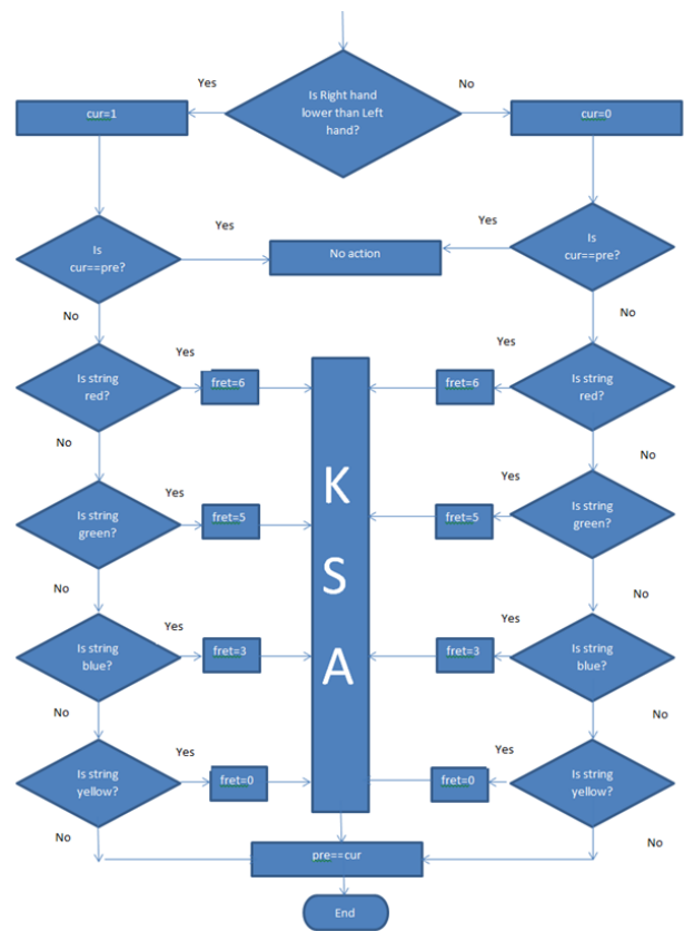
Figure 3. Project Flowchart- Part two
