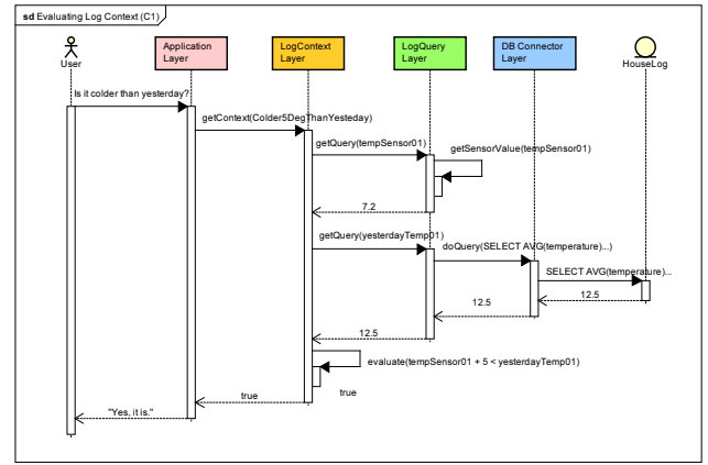
Figure 3: Sequence diagram for evaluating log context (C1) “it is 5 degree colder than yesterday.”
