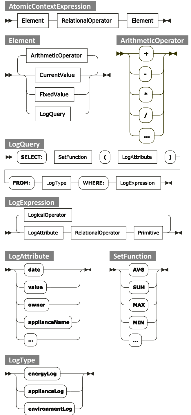
Figure 2: Syntax diagram of context expression (extended version).
