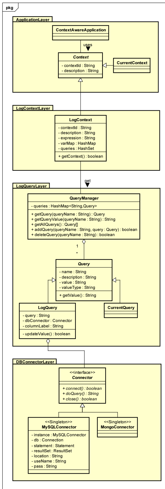
Figure 4: Class diagram of the developed system.
