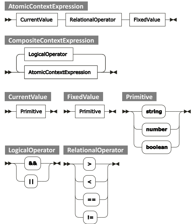
Figure 1: Syntax diagram of context expression (original version).
