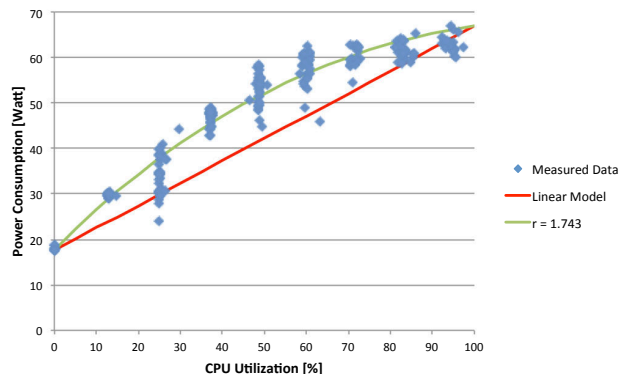
Figure 1: Power consumption models vs utilization
