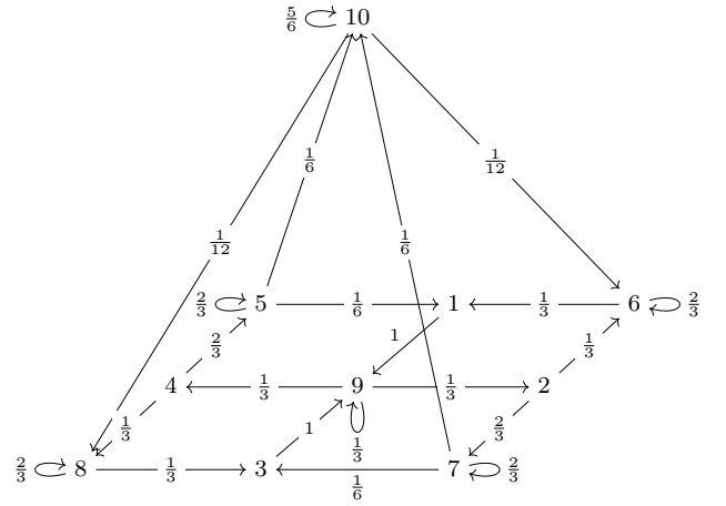
Figure 5: Reversed chain of the DTMC in Figure 4
