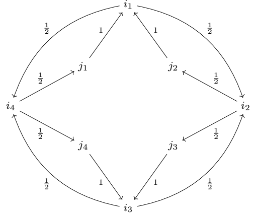
Figure 2: Reversed chain of the DTMC in Figure 1
