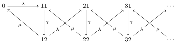
Figure 6: Infinite state space CTMC.
