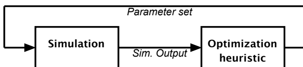
Figure 1: Common black-box optimization, see [2]
